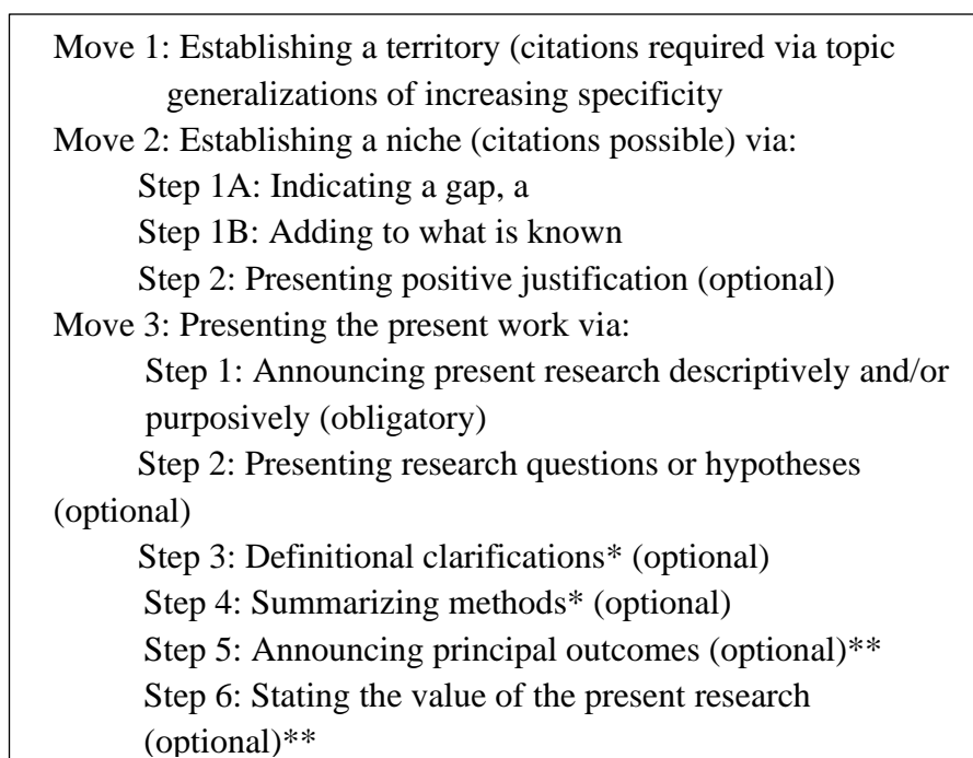
Figure 1. Swales' (2004, p. 230, 232) create a research space model
