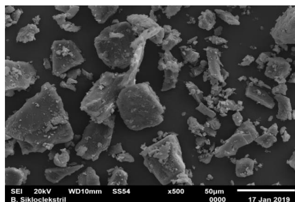
\beta -cyclodextrin
