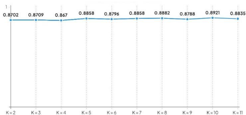
Figure 4. K-fold experiment
