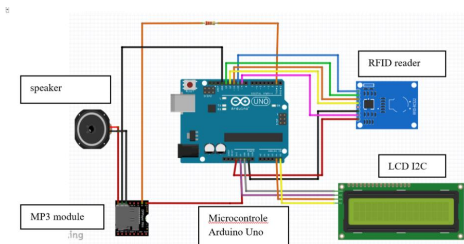
Figure 3. The main electrical circuit of the prototype
