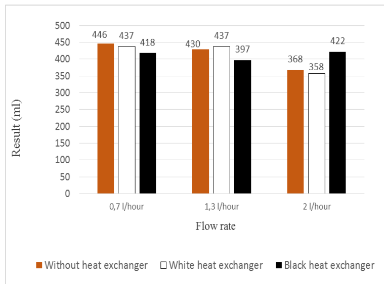
Figure 3. Graph of results of indoor distillation data
