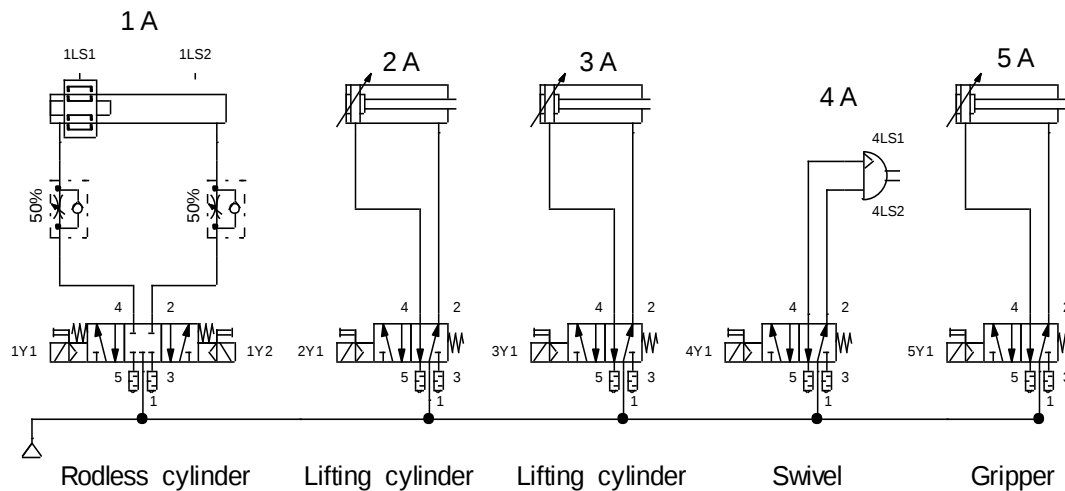
Figure 3. Pneumatic circuit
