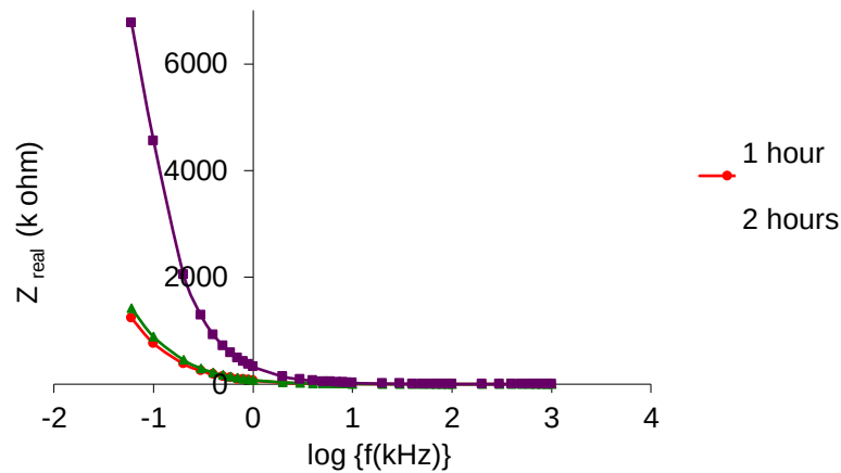
Figure 1. Graph of Z_{\text{real}} vs log frequency (annealed at 900°C for 1 hour, 2 hours and 4 hours)
