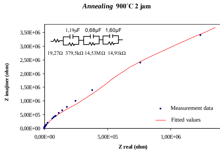
Figure 5. Comparison of measurement data & the results of fitting on samples annealed at 900°C for 2 hours
