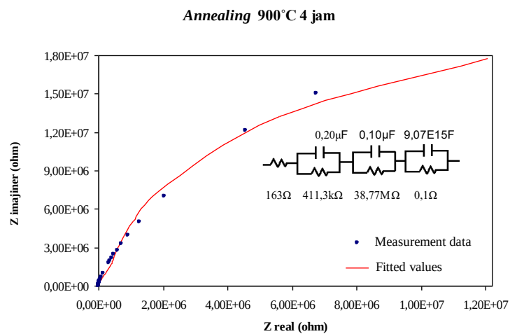
Figure 6. Comparison of measurement data & the results of fitting on samples annealed at 900°C for 4 hours
